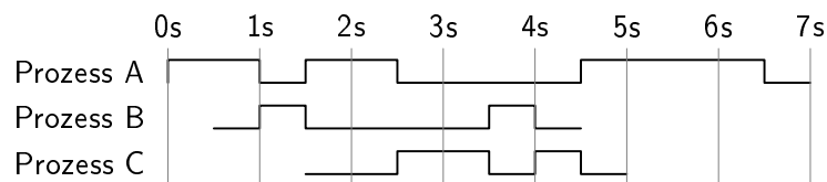
Abbildung 1: Round-Robin Scheduling
